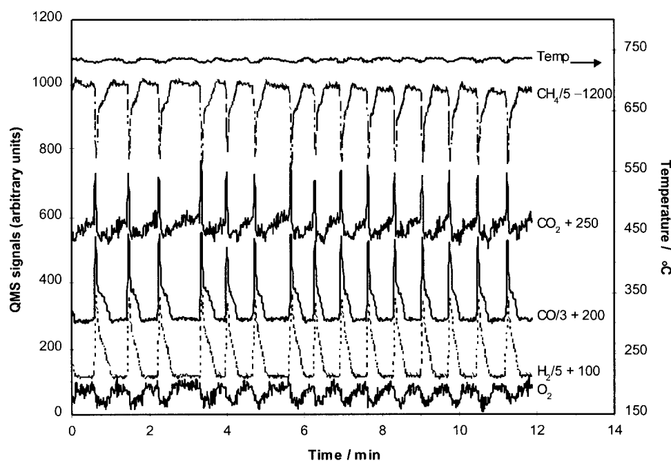
Figure 6. Oscillations observed over a nickel wire. (Ni wire, 20 cm long, 0.25 mm diameter; Ar : CH 4 : O 2 = 30 : 29.5 : 0.5 ml min -1 , system temperatures 730 °C.)
